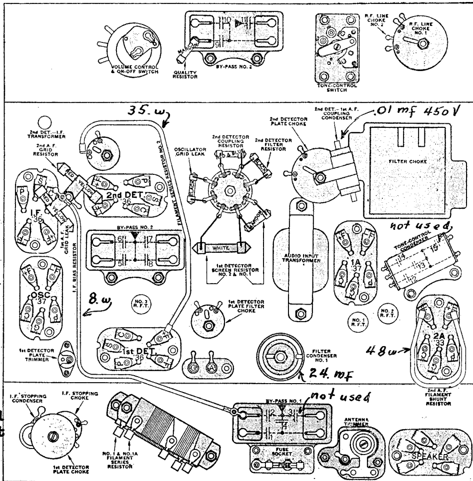
BOTTOM CHART.
